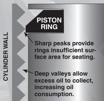
Fig. 1: New Cylinder
