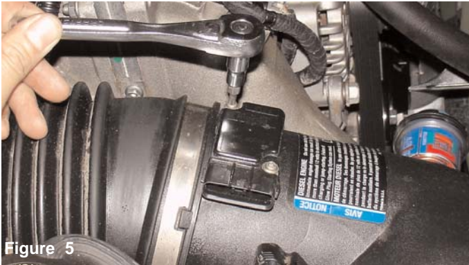
Figure 5 Use the T20 torx bit to loosen and remove the bolts on the mass air flow sensor.
