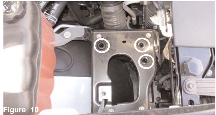
Figure 10 The pegs on the air box mounting plate are designed to be inserted into the three stock grommets that are circled above.
